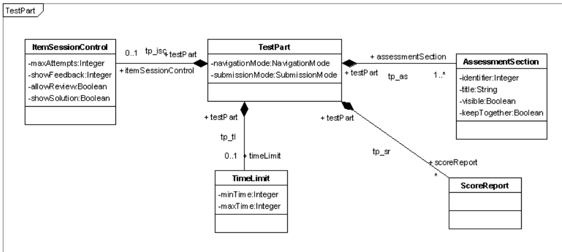
Figure 9: TestPart Metaclass
