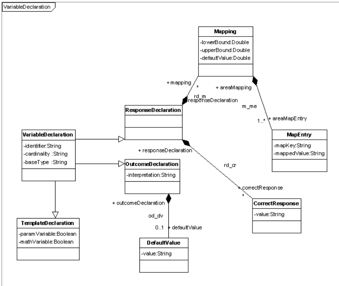
Figure 2: VariableDeclaration Metaclass
