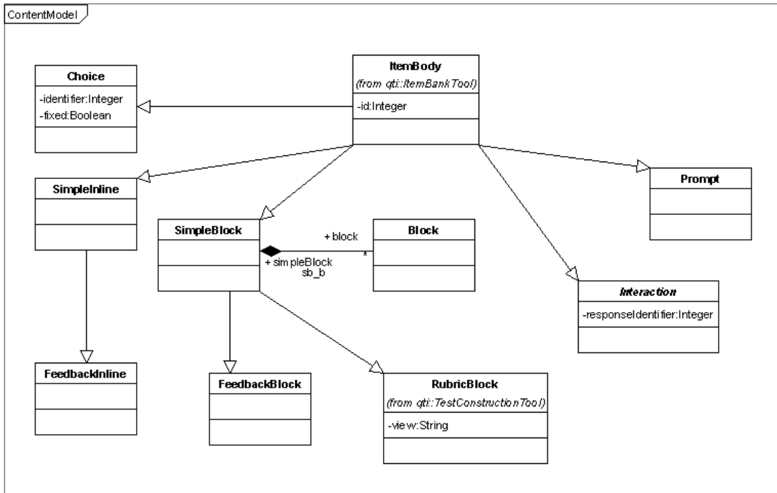
Figure 4: ItemBody Metaclass
