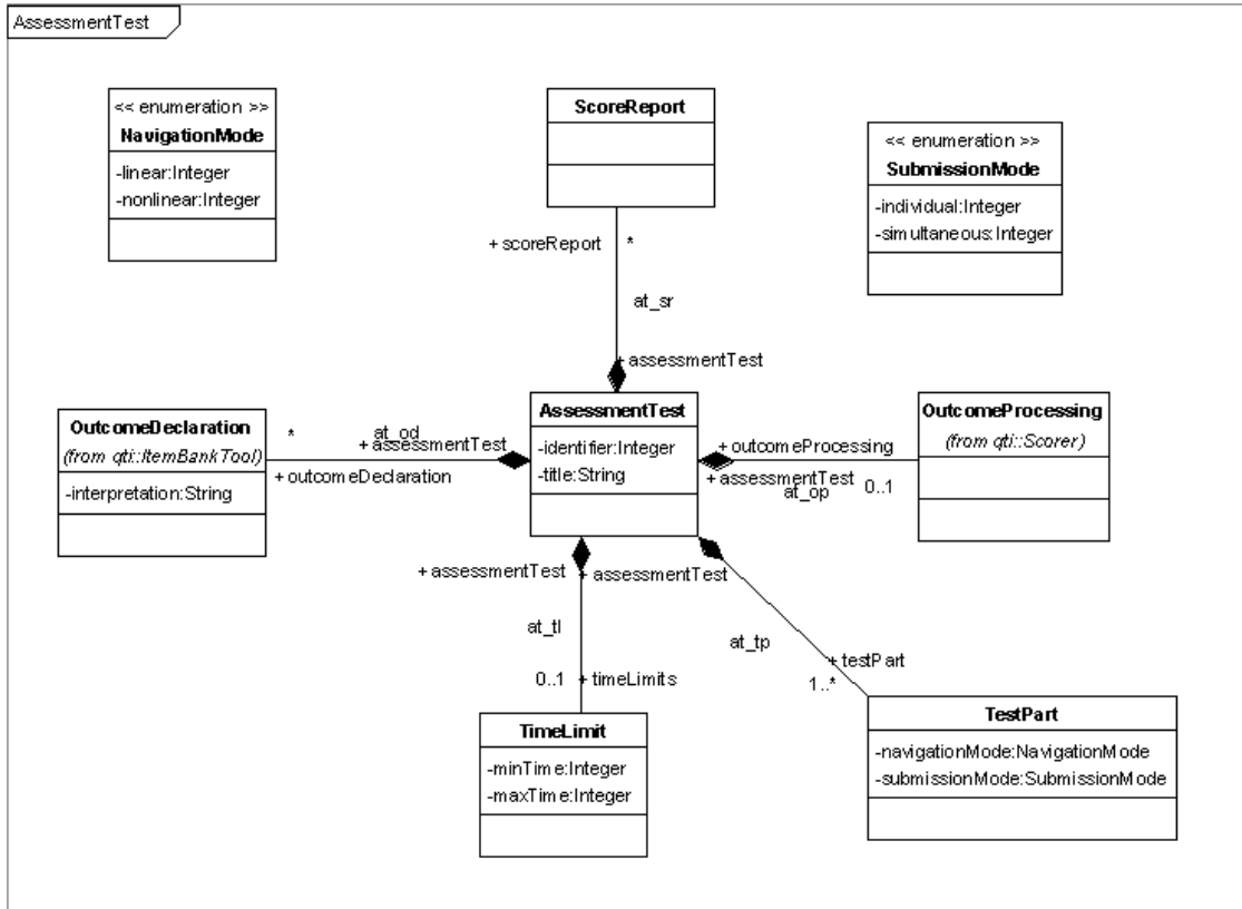
Figure 8: AssessmentTest Metaclass
