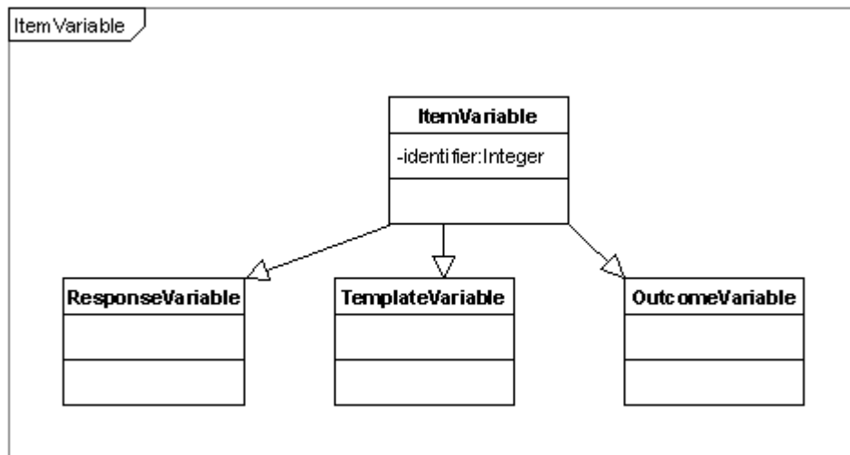
Figure 3: ItemVariable Metaclass
