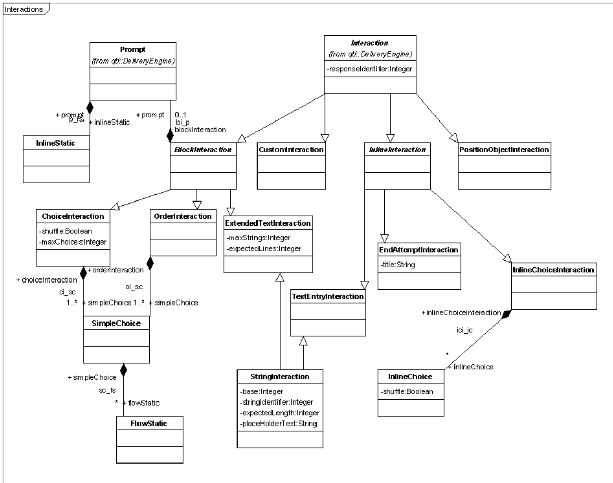
Figure 6: Interaction Metaclass
