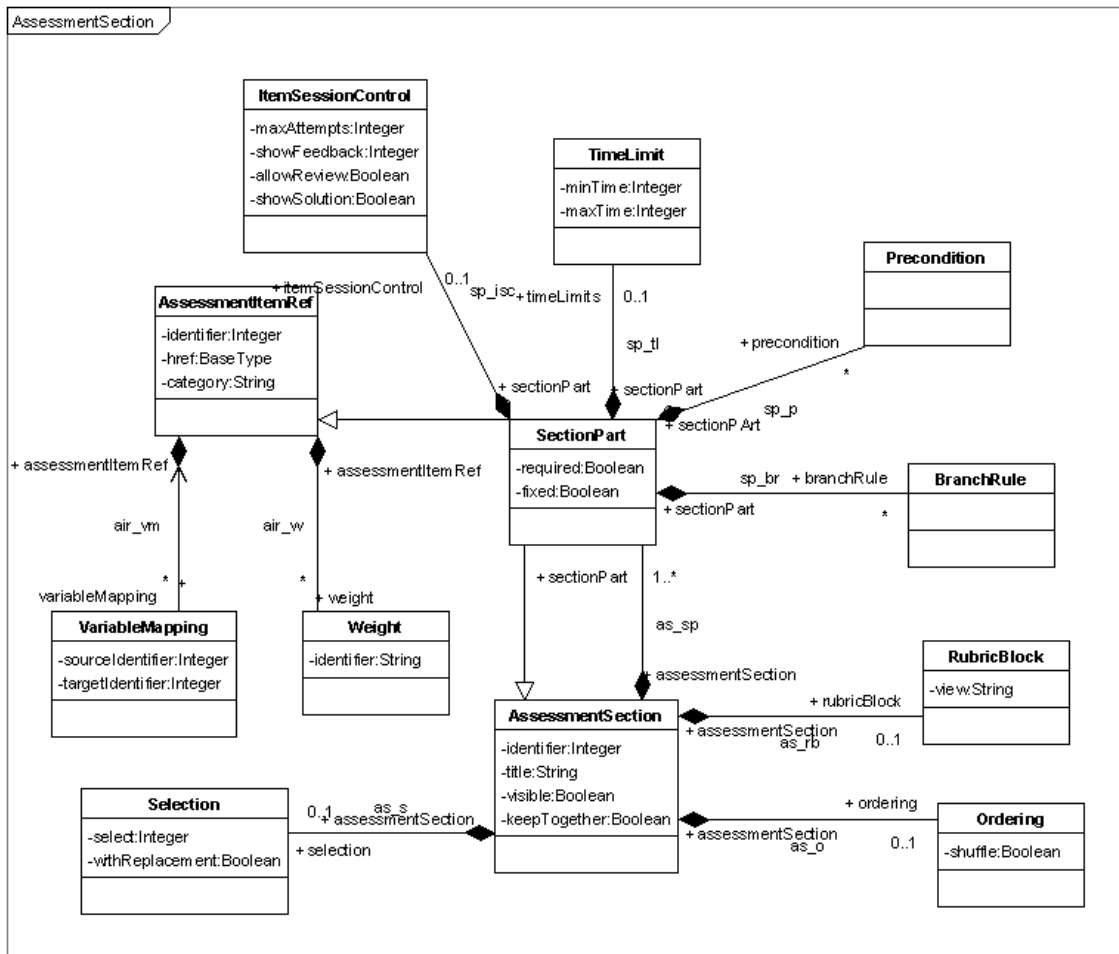
Figure 10: AssessmentSection Metaclass
