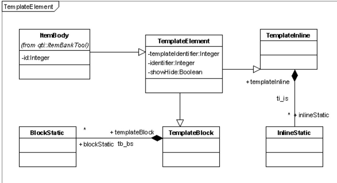
Figure 5: TemplateElement Metaclass
