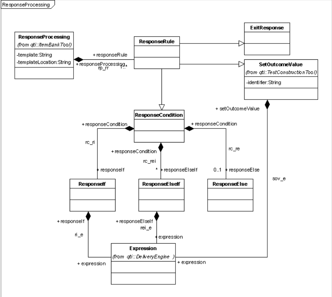
Figure 12: ResponseProcessing Metaclass
