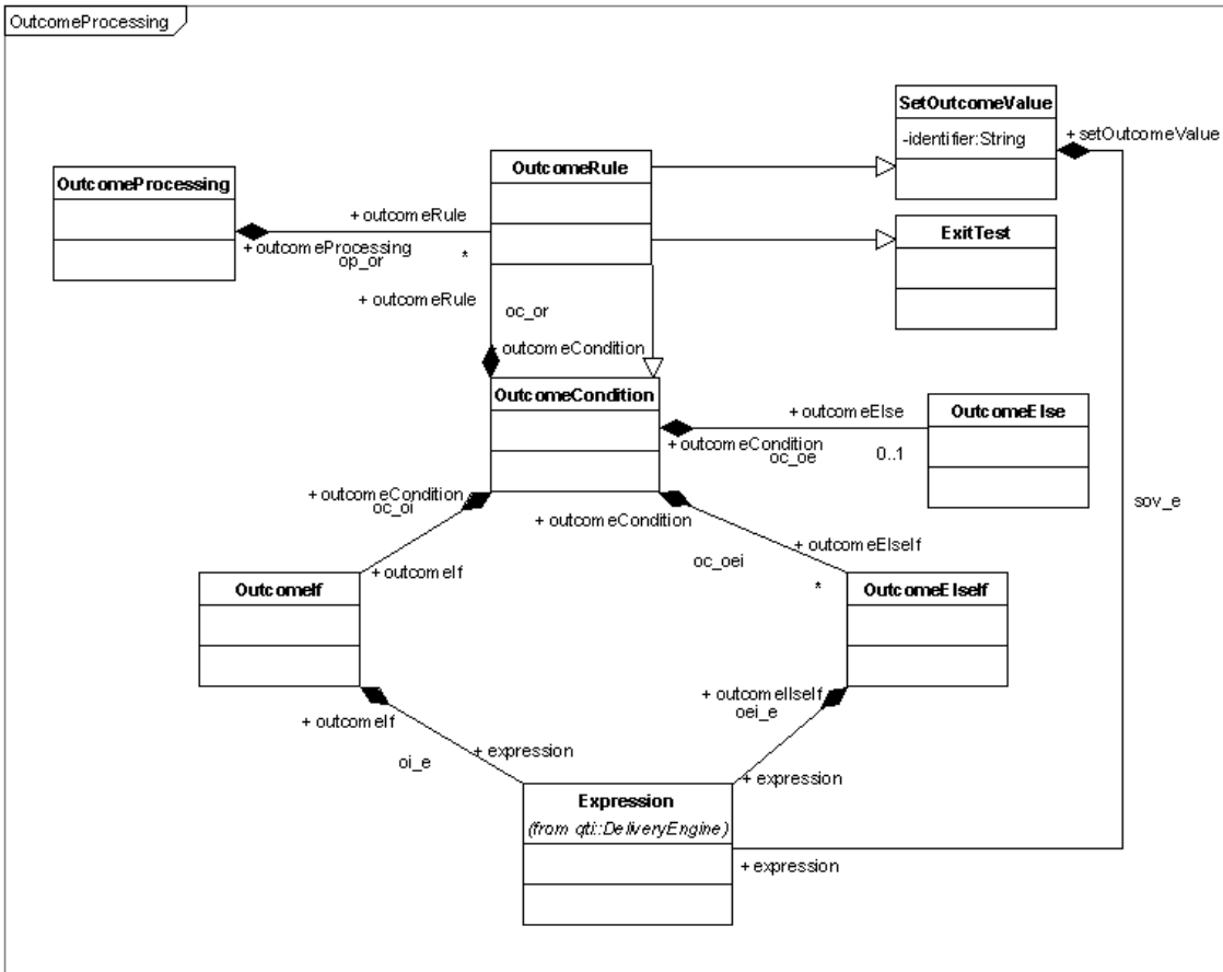
Figure 11: Outcome Processing
