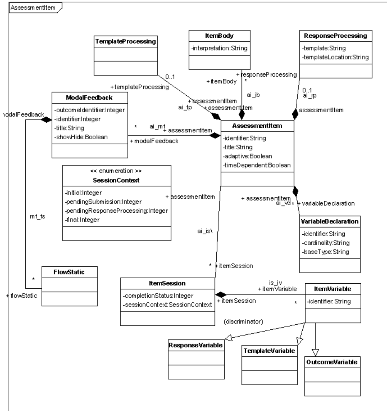
Figure 1: AssessmentItem Metaclass
